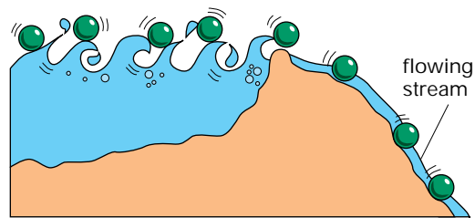
catalyzed reaction—waves often surmount barrier
