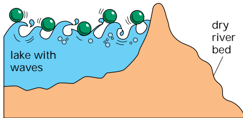
uncatalyzed reaction—waves not large enough to surmount barrier
